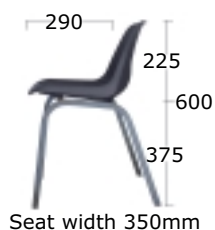
G5 PRIMARY POLYSHELL CHAIR HEIGHT: 375mm COLOURS: Red or Blue Open Back. Charcoal, Red or Blue Closed Back
