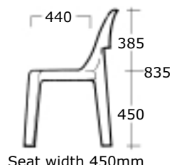
G3 ALPINE CHAIR HEIGHT: 450mm COLOURS: Red, White, Blue, Green, Hunter's Green, Beige, Brown, Yellow, Burgundy, Charcoal, Black
